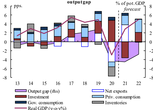
Graph II.3.1: Estonia - Real GDP growth and contributions, output gap
