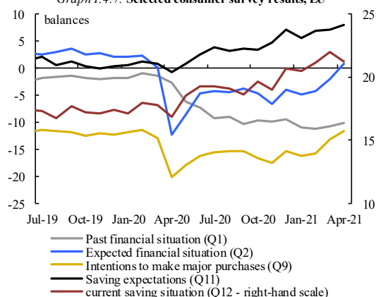
Graph I.4.7: Selected consumer survey results, EU
