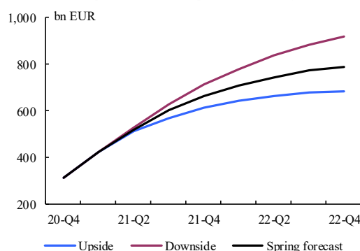
Graph I.4.3: Model-implied excess savings
