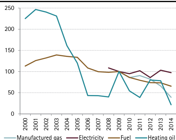
Figure I: Index of physical energy consumption per output (2009=100)
